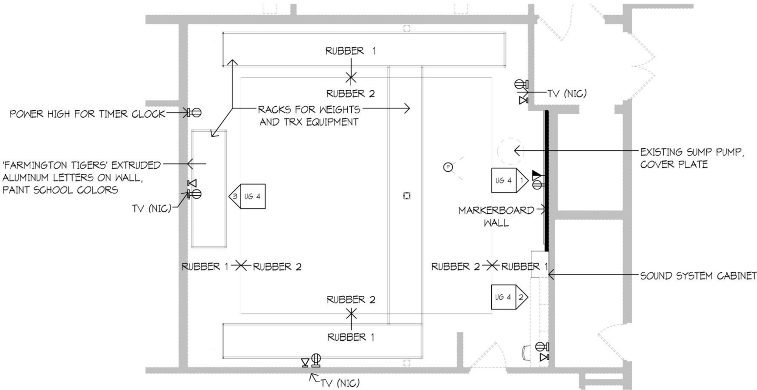
1 FARMINGTON HS FLEX ATHLETIC ROOM 1/8" = 1'-0" 0 6' 12'
