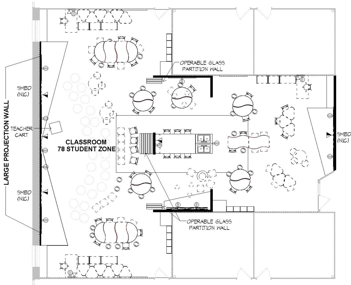
1 AKIN ROAD LARGE GROUP LAYOUT 1/8" = 1'-0"
