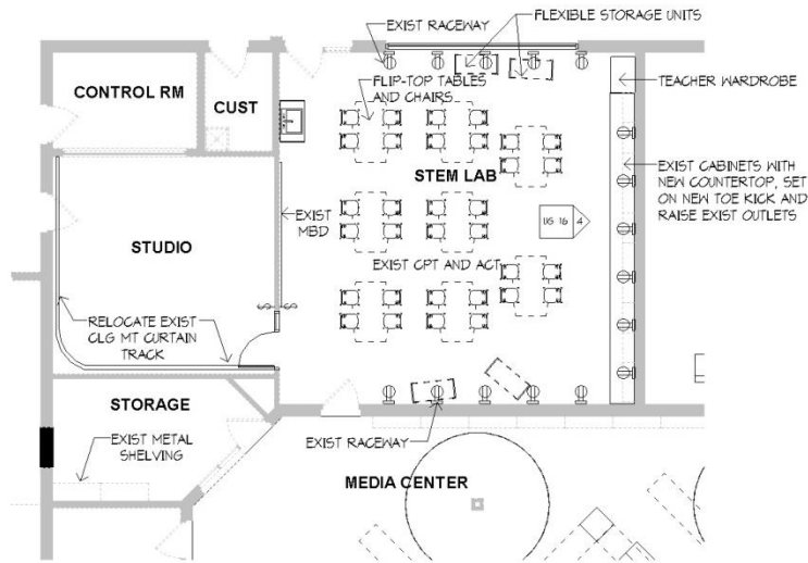
1 MEADOWVIEW ES STEM LAB 1/8" = 1'-0"
