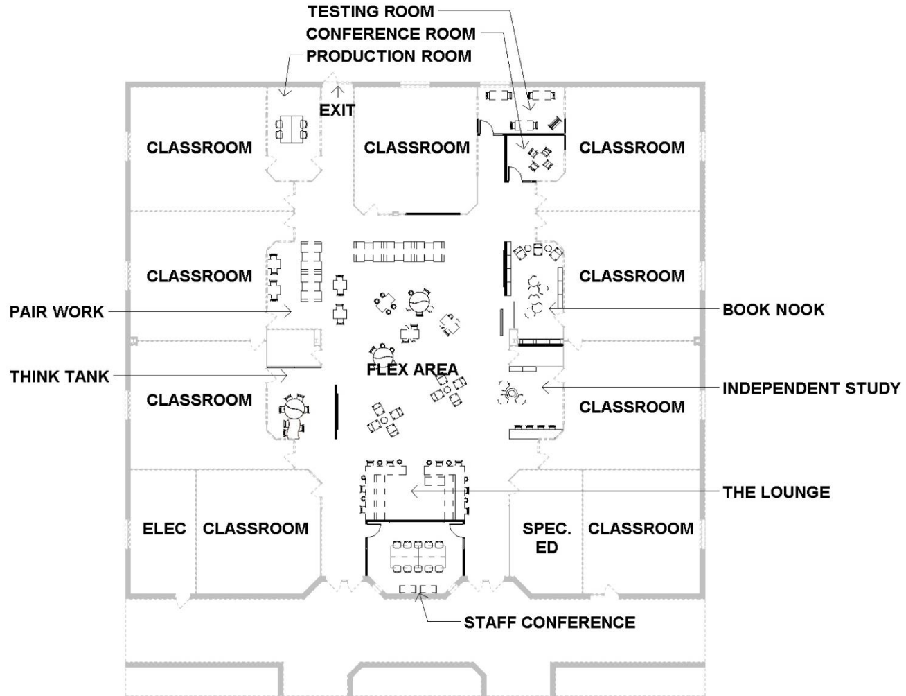
1 BOECKMAN MS OVERALL PLAN 3/64" = 1'-0" 0 16' 32'
